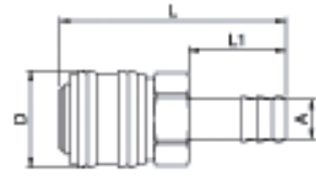
Hose connection
